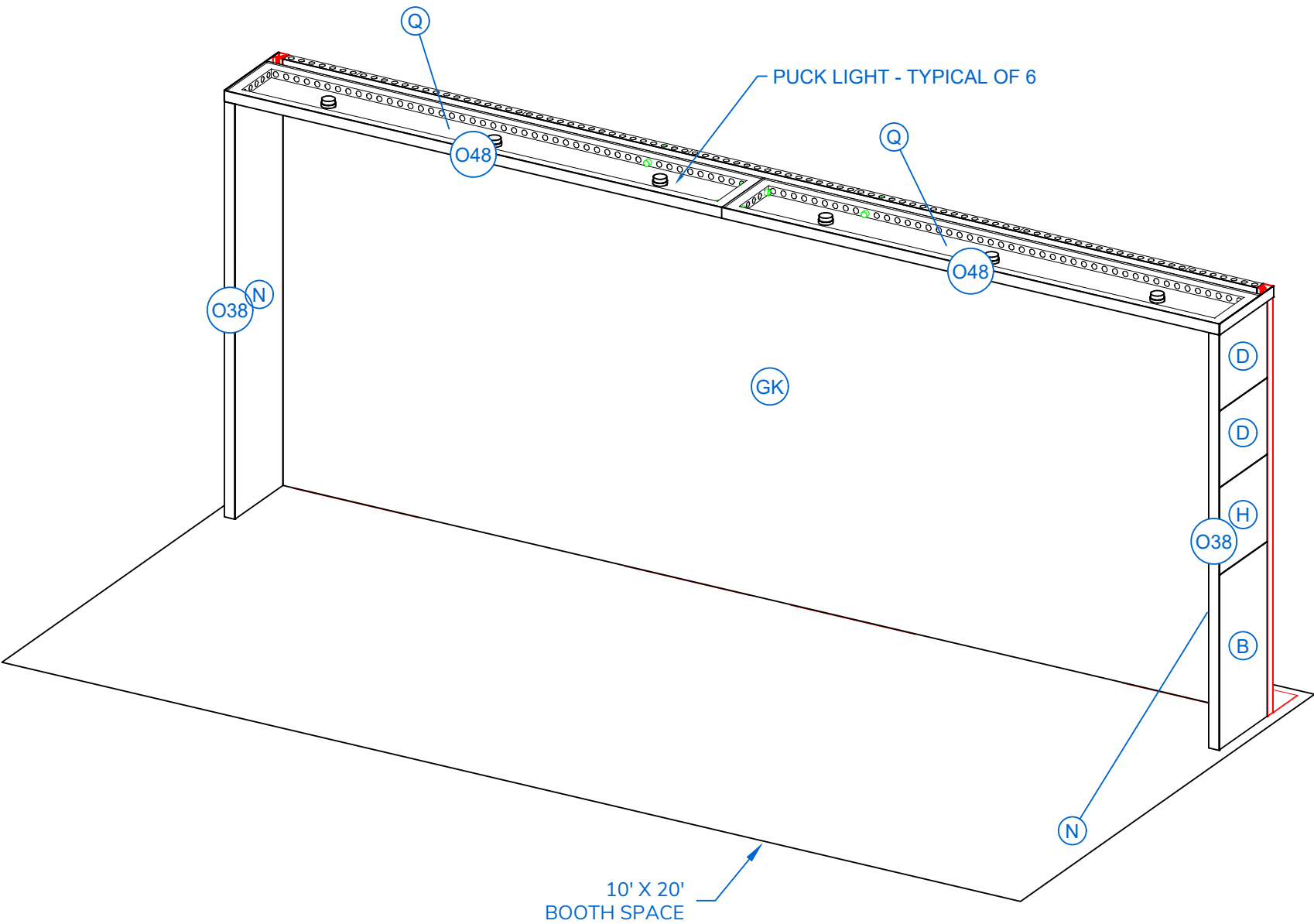
3D VIEW: STRUCTURE FRONT
