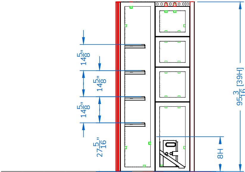
ELEVATION F - COVERINGS REMOVED TO SHOW SHELF HEIGHTS
