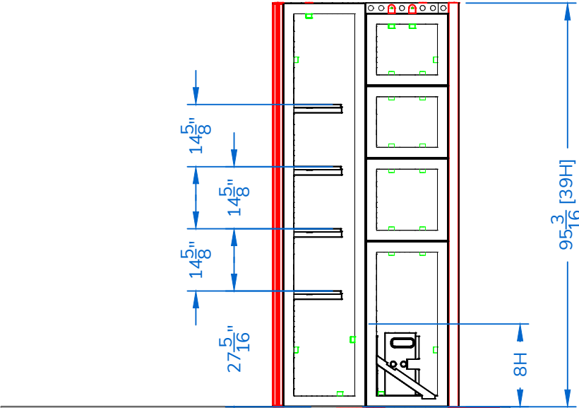
ELEVATION B - COVERINGS REMOVED TO SHOW SHELF HEIGHTS
