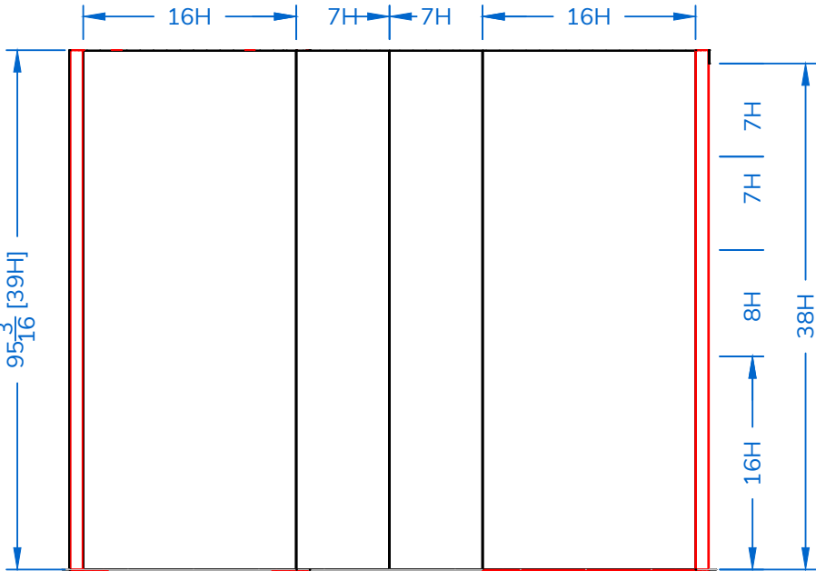
ELEVATION C
