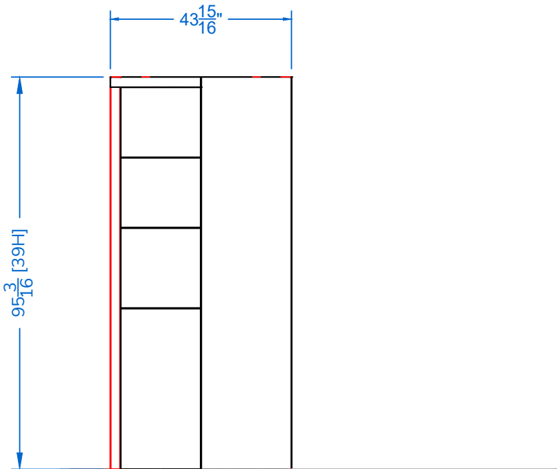
ELEVATION F - COVERINGS REMOVED TO SHOW SHELF HEIGHTS
