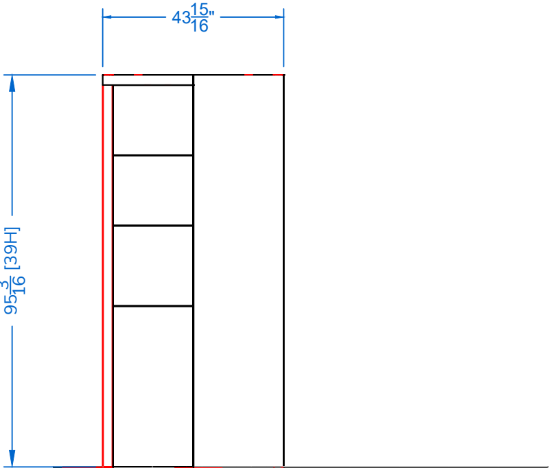
ELEVATION B - COVERINGS REMOVED TO SHOW SHELF HEIGHTS
