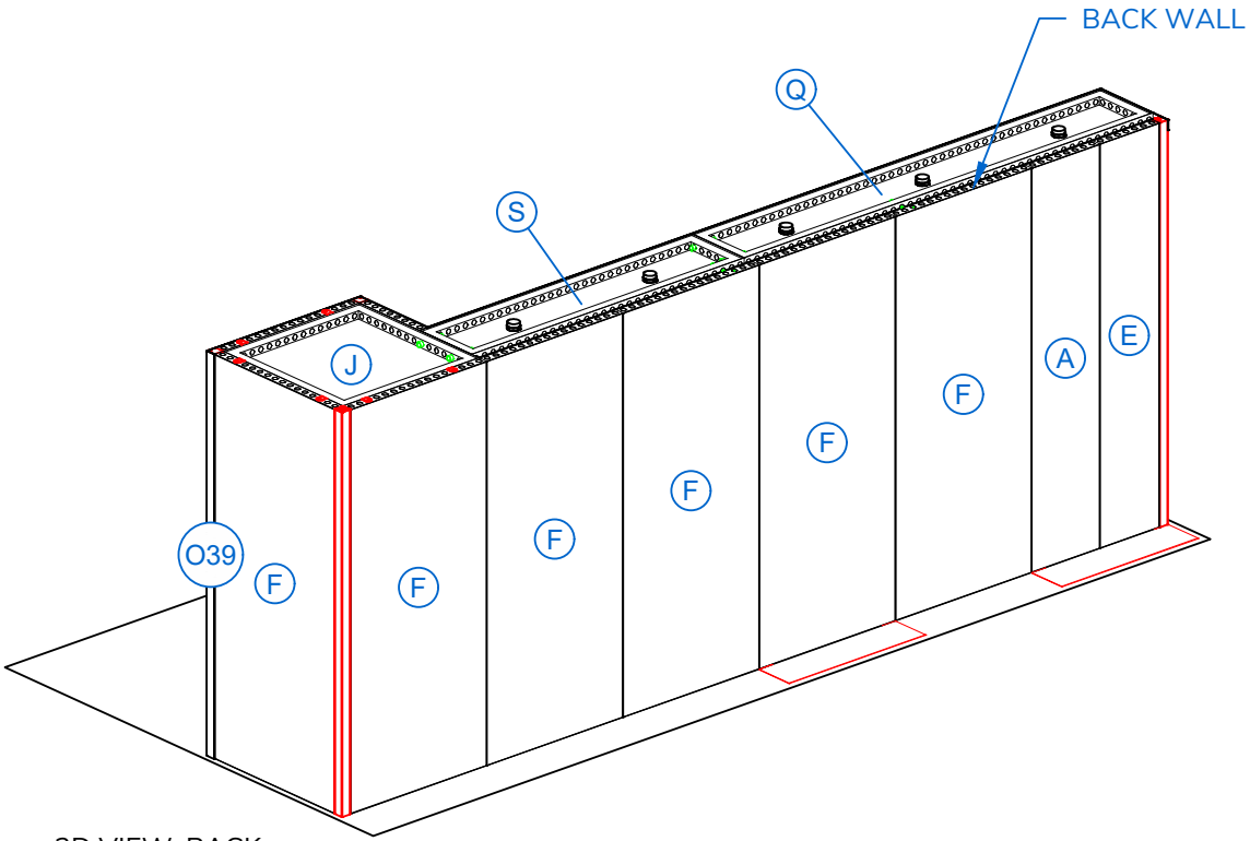
3D VIEW: BACK
