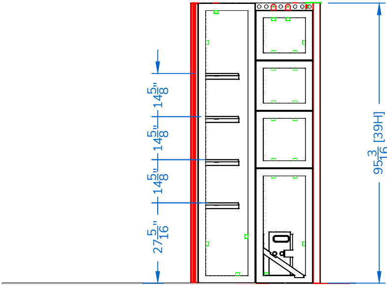
ELEVATION B - COVERINGS REMOVED TO SHOW SHELF HEIGHTS
