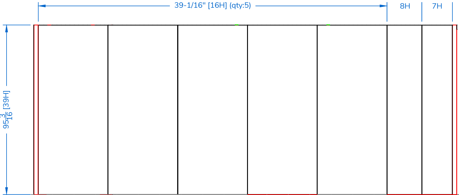
ELEVATION C
