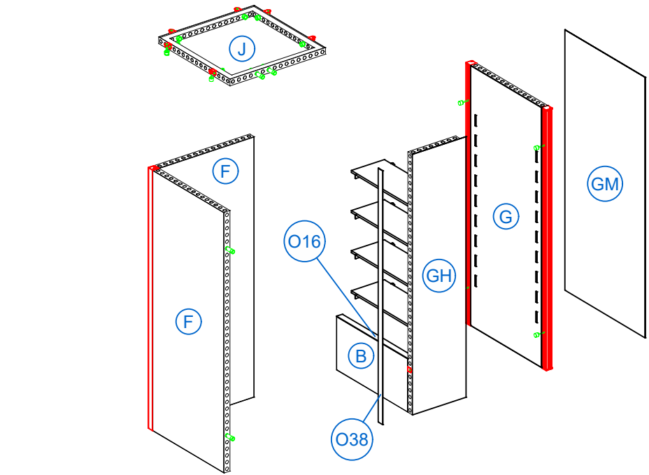
3D VIEW: EXPLODED VIEW - SHELVES
