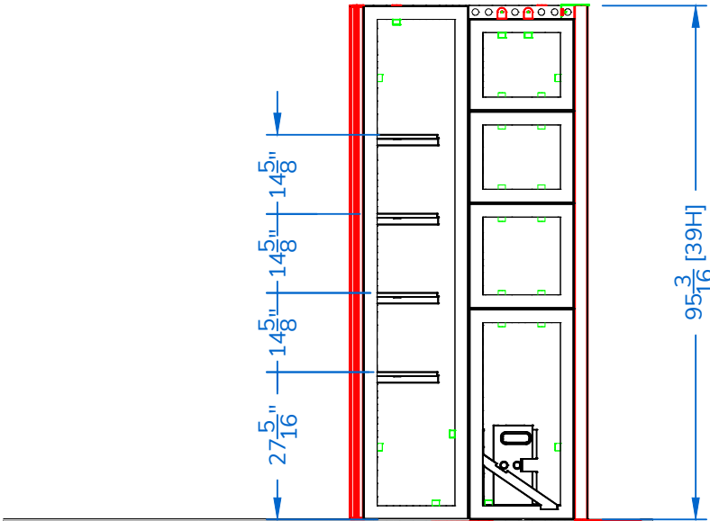
ELEVATION F - COVERINGS REMOVED TO SHOW SHELF HEIGHTS
